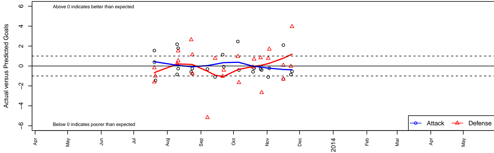
United FC White B00 Dots are actual minus expected GF (blue circles) and GA (red triangles). Blue line is smoothed change in attack strength. Red is smoothed change in defense strength.
